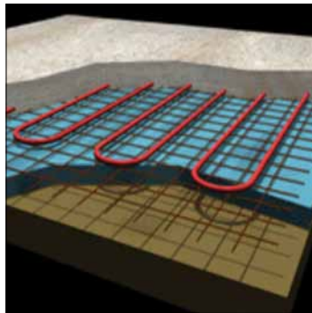
Radiant floor heating and snow and ice melt applications
