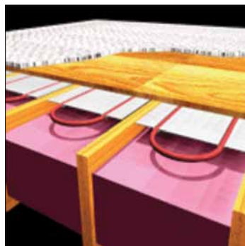
Under or over the floor radiant systems with heat transfer plates
